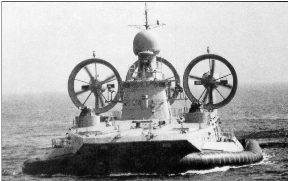
Figure 10. The Former USSR Pomornik Military ACV
