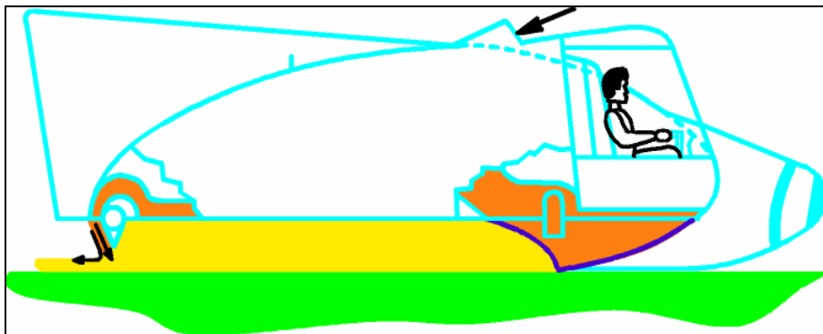
Figure 3. Flexible Bow Seal by Beardsley, USA, 1957
