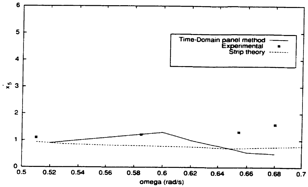
Figure 4.108: Computed pitch for F_n = 0.15 , 2l_y/B = 1.04
