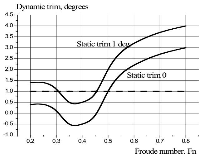
Figure 1 Typical dependence of the SWATH trim on the length Froude number, with positive and zero static trim (positive trim corresponds to bow up)
