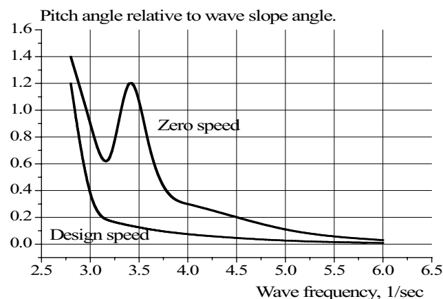
Figure 9 Response amplitude operator of pitch in head waves
