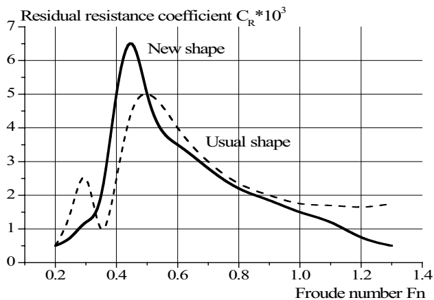
Figure 7 Residual resistance coefficient of the model tested at two draughts
