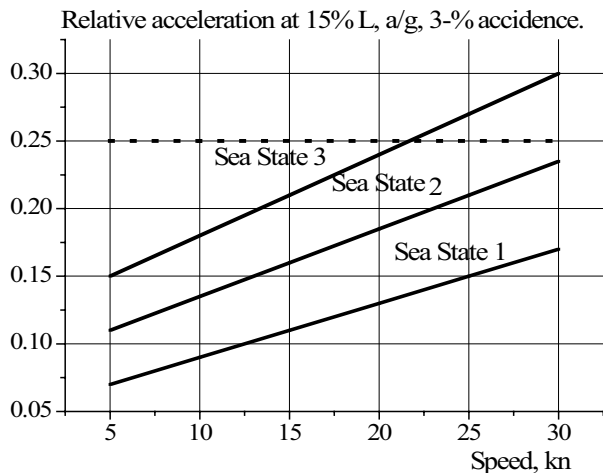
Figure 12 Relative vertical acceleration a/g at 15%L from FP, 3% accident
