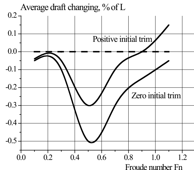
Figure 3 Example of the mean dynamic draught variation of a SWATH
