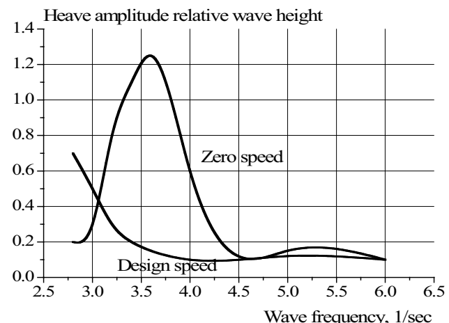
Figure 10 Response amplitude operator of heave in head waves
