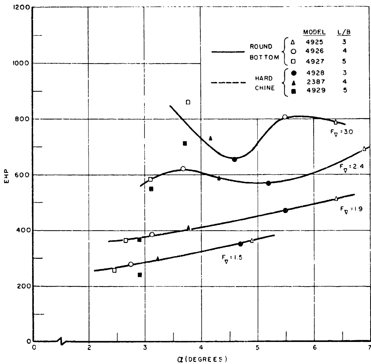
FIGURE 11A. EHP VERSUS \alpha IN CALM WATER
