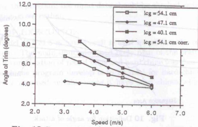
Fig. 12 Computed trim/speed for displacement 18.9 kg
