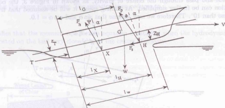
Fig. 1 Hydrodynamic and static forces on a planing hull
