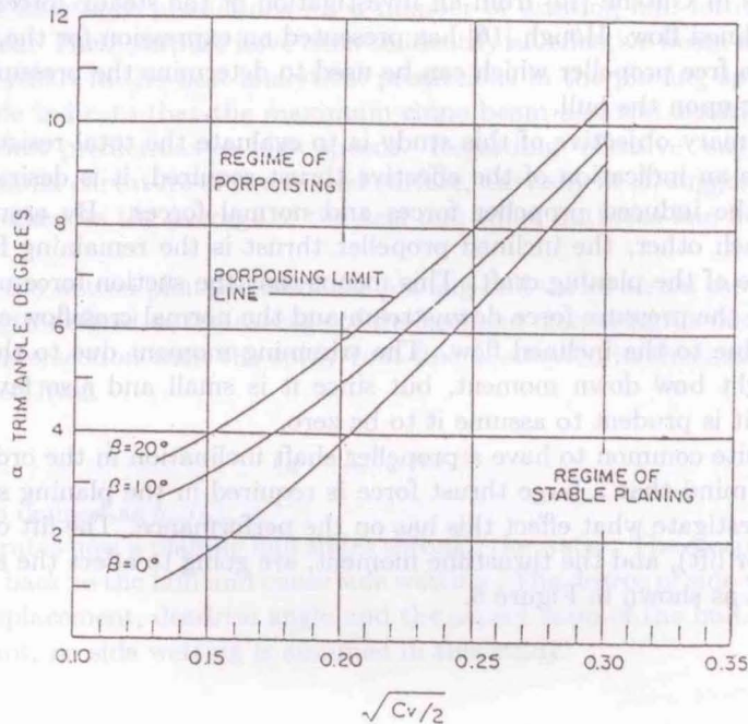
Fig. 7 Relationship between trim angle and lift coefficient [8]
