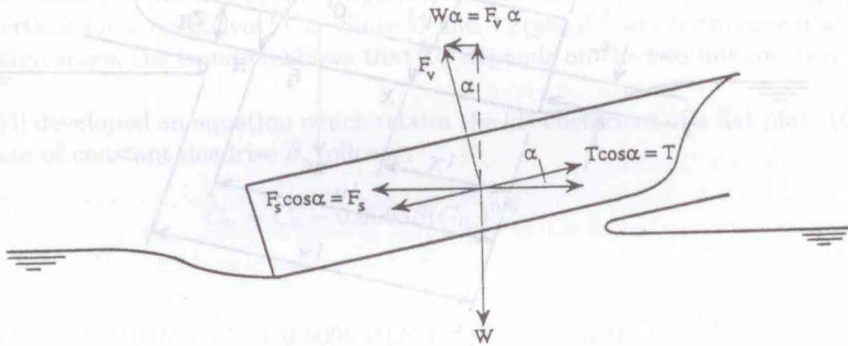
Fig. 3 Simplified force diagram
