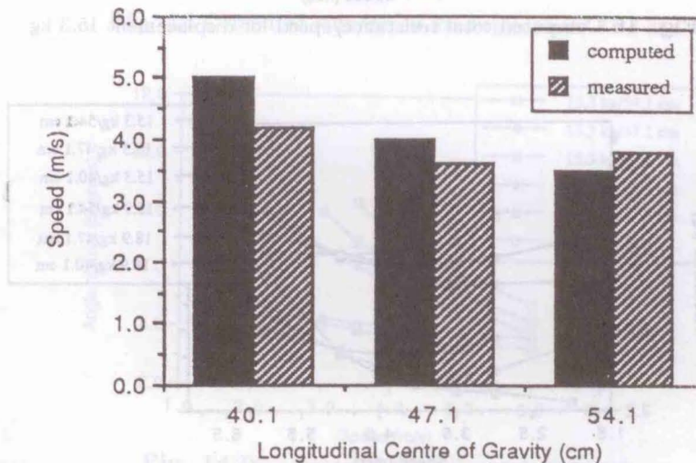
Fig. 18 Start of planing for displacement 18.9 kg
