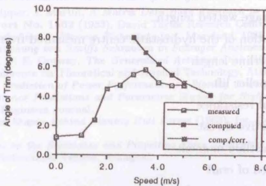
Fig. 31 Angle of trim/speed for displacement 18.9 kg and leg 40.1 cm
