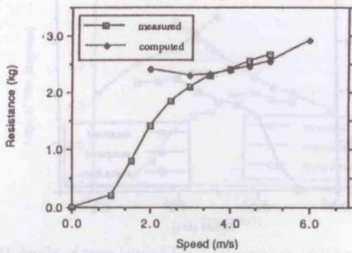
Fig. 24 Total resistance/speed for displacement 18.9 kg and leg 47.1 cm
