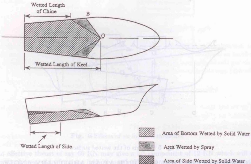
Fig. 4 Geometry of the wetted surface
