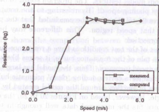
Fig. 22 Total resistance/speed for displacement 18.9 kg and leg 40.1 cm
