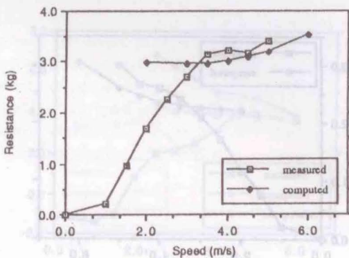
Fig. 20 Total resistance/speed for displacement 18.9 kg and leg 54.1 cm
