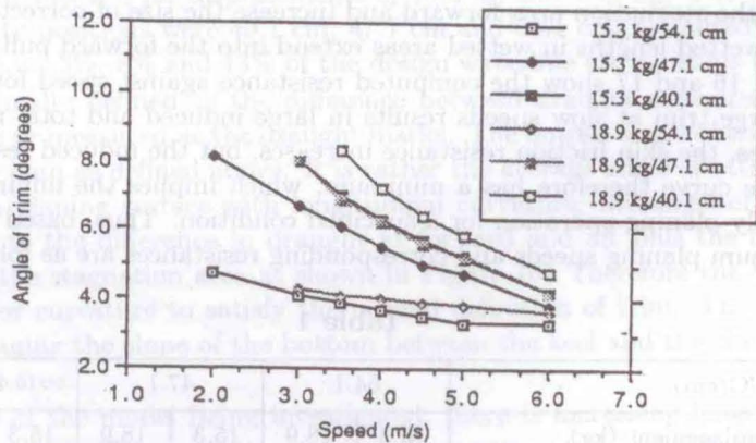
Fig. 14 Trim corrected for hull curvature/speed
