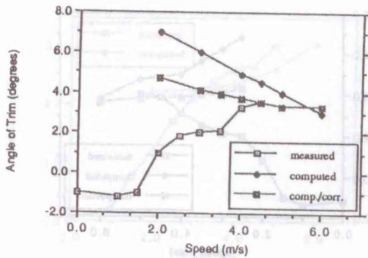
Fig. 29 Angle of trim/speed for displacement 18.9 kg and leg 54.1 cm
