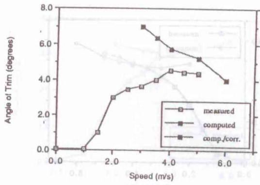
Fig. 27 Angle of trim/speed for displacement 18.9 kg and leg 47.1 cm
