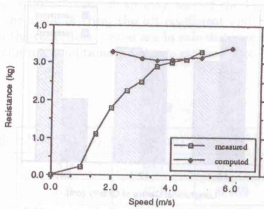
Fig. 21 Total resistance/speed for displacement 18.9 kg and leg 47.1 cm
