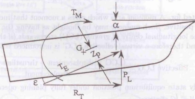
Fig. 6 Effects of an inclined thrustline
