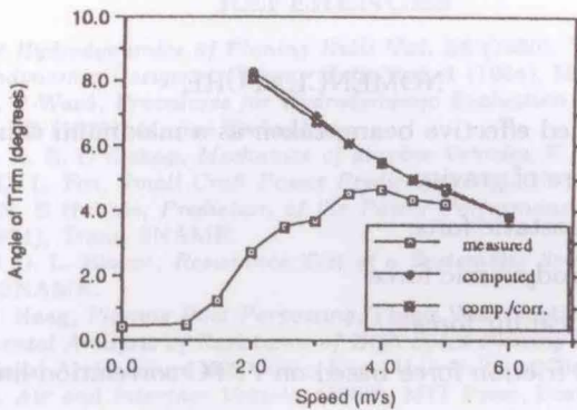
Fig. 30 Angle of trim/speed for displacement 18.9 kg and leg 47.1 cm
