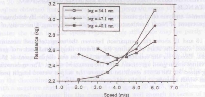
Fig. 16 Computed total resistance/speed for displacement 15.3 kg
