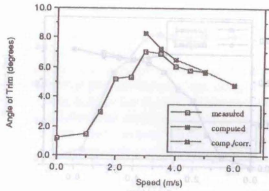
Fig. 28 Angle of trim/speed for displacement 18.9 kg and leg 40.1 cm
