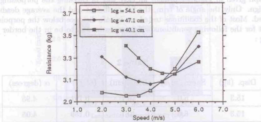
Fig. 15 Computed total resistance/speed for displacement 18.9 kg
