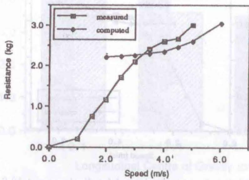
Fig. 23 Total resistance/speed for displacement 18.9 kg and leg 54.1 cm
