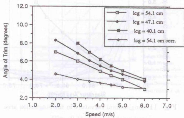
Fig. 13 Computed trim/speed for displacement 15.3 kg
