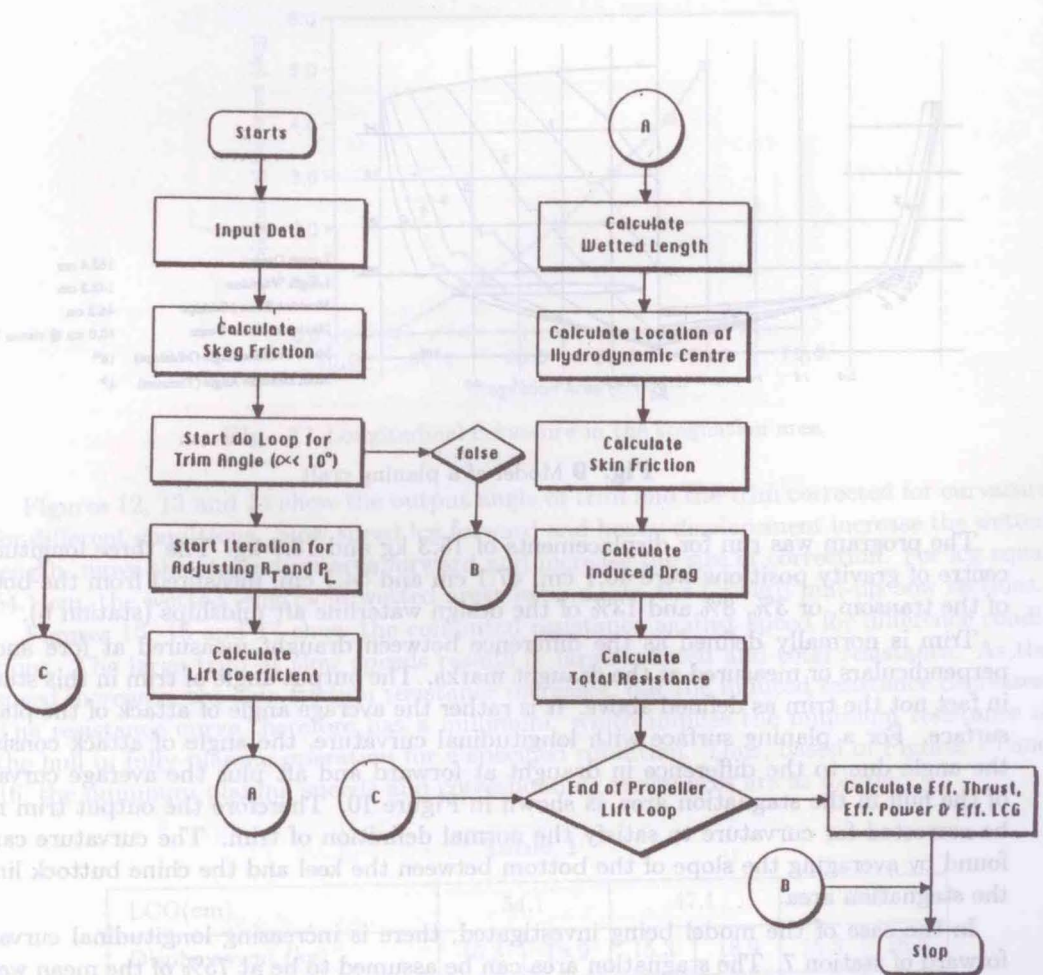
Fig. 8 Computer flowchart for resistance prediction
