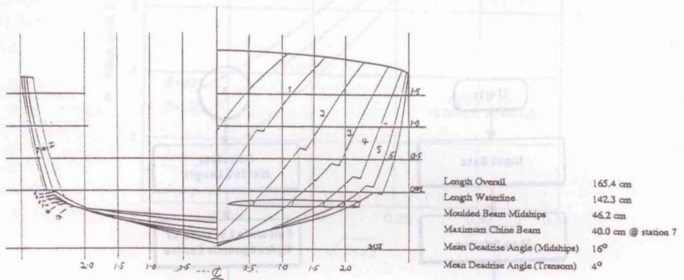
Fig. 9 Model of a planing craft
