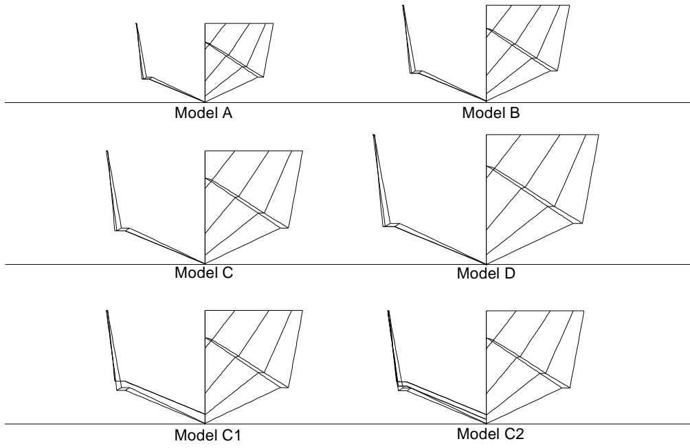
Figure 1: Model body plans.
