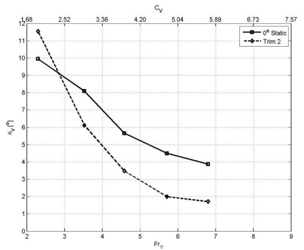
Figure 18: Model B – dynamic trim [trim 1 was produced by a 4.74Nm shift in ballast towards the stern. Trim 2 was produced by a 9.89Nm shift in ballast towards the stern.]
