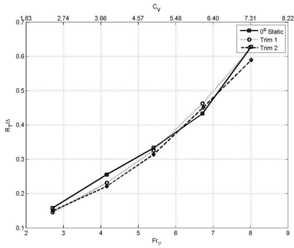
Figure 5: Model A – resistance [trim 1 was produced by a 2.94Nm shift in ballast towards the stern. Trim 2 was produced by a 6.87Nm shift in ballast towards the stern.]
