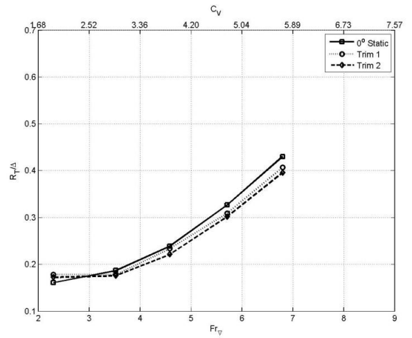
Figure 8: Model D – resistance [trim 1 was produced by a 10.20Nm shift in the ballast towards the stern. Trim 2 was produced by a 20.01Nm shift in the ballast towards the stern.]
