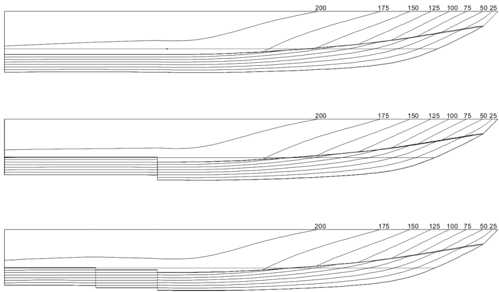
Figure 2: Model profiles (model A-D, model C1, model C2). [Buttock lines in mm]
