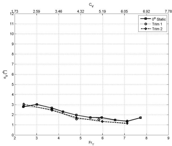
Figure 17: Model A – dynamic trim [trim 1 was produced by a 2.94Nm shift in ballast towards the stern. Trim 2 was produced by a 6.87Nm shift in ballast towards the stern.]
