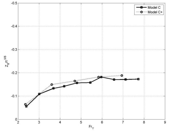
Figure 38: Influence of load coefficient on dynamic sinkage
