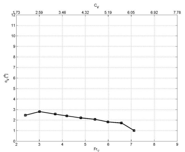
Figure 22: Model C2 – dynamic trim
