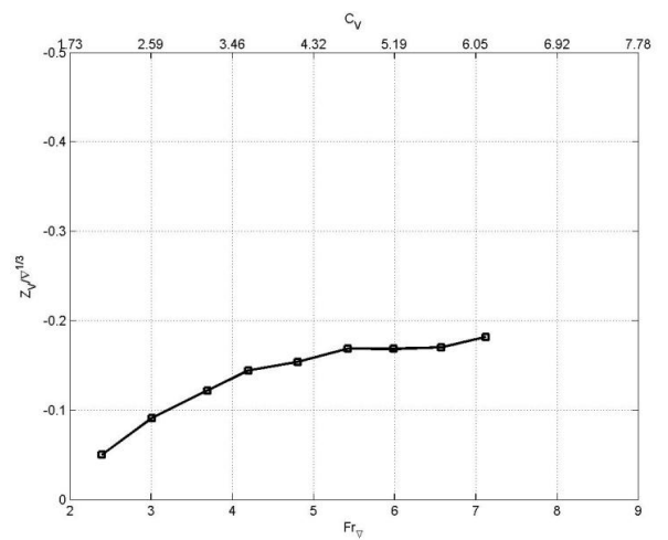
Figure 16: Model C2 – dynamic sinkage
