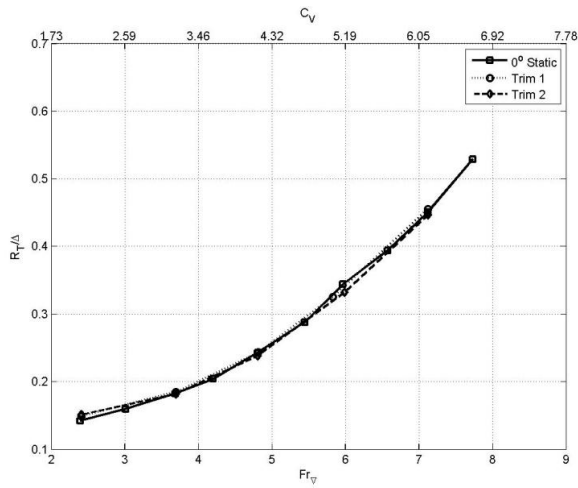
Figure 7: Model C – resistance [trim 1 was produced by a 7.85Nm shift in ballast towards the stern. Trim 2 was produced by a 14.72Nm shift in ballast towards the stern.]
