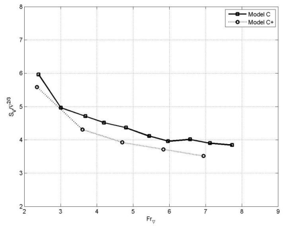
Figure 40: Influence of load coefficient on wetted surface area
