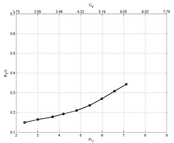
Figure 10: Model C2 - resistance
