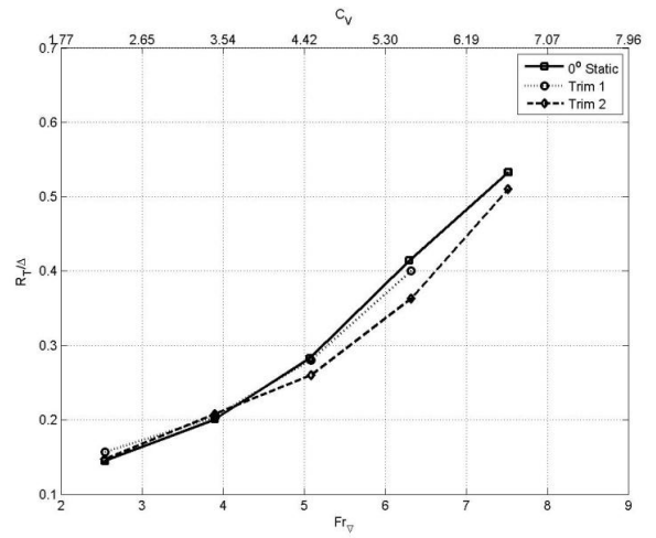
Figure 6: Model B – resistance [trim 1 was produced by a 4.74Nm shift in ballast towards the stern. Trim 2 was produced by a 9.89Nm shift in ballast towards the stern.]
