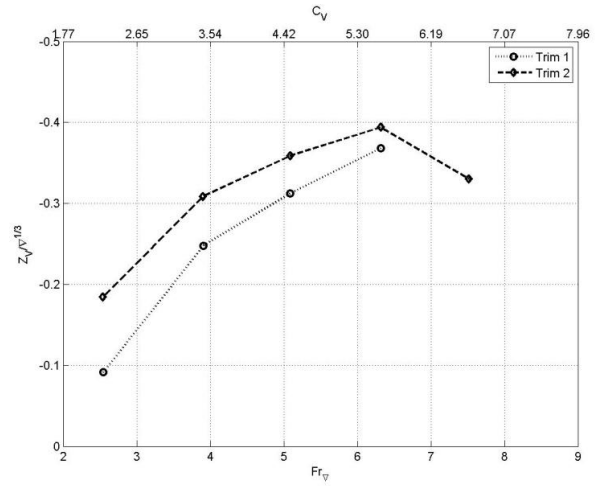
Figure 12: Model B – dynamic sinkage [trim 1 was produced by a 4.74Nm shift in ballast towards the stern. Trim 2 was produced by a 9.89Nm shift in ballast towards the stern.]
