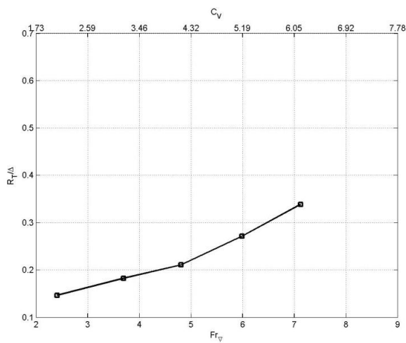
Figure 9: Model C1 - resistance
