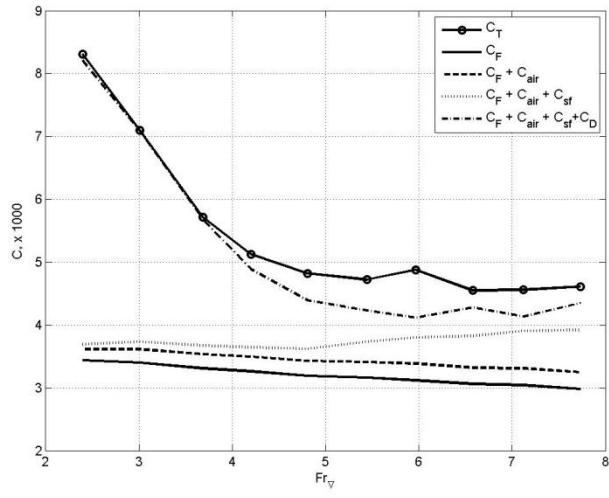
Figure 41: Model C - resistance coefficients
