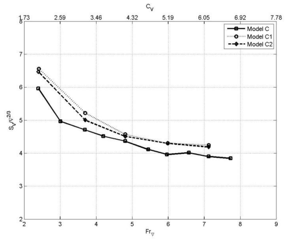
Figure 36: Influence of transverse steps on wetted surface area
