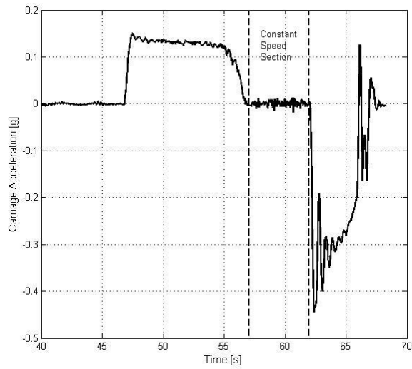
Figure 3: Example carriage acceleration record (for a carriage speed of 12.05 m/s).
