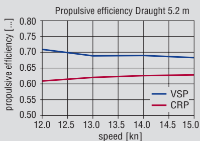
Diagram 4: Propulsive efficiency/ Draught 5.2 m
