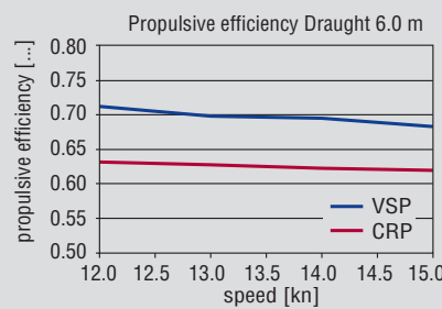
Diagram 5: Propulsive efficiency/ Draught 6.0 m
