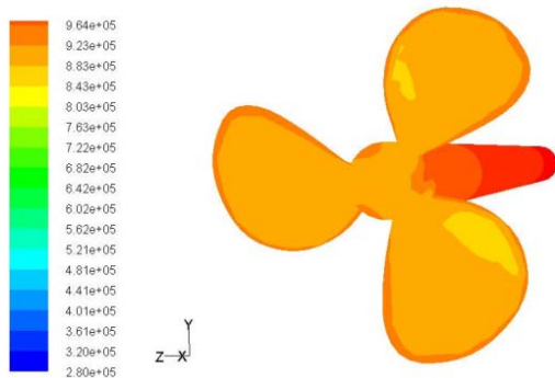
Figure 7: Flow pressure contour (pa) ( V_a=3\text{m/s} , N=120\text{rpm} ).
