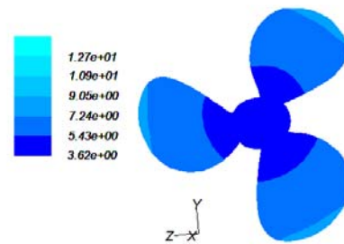
Figure 10: Flow velocity contour (m/s) ( V_a=5\text{m/s} , N=250\text{rpm} ).
