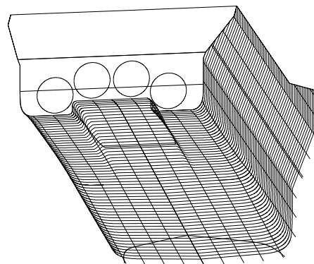
Figure 7 – Containership Gully Stern Arrangement
