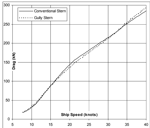
Figure 14 - RT Vs Ship Speed
