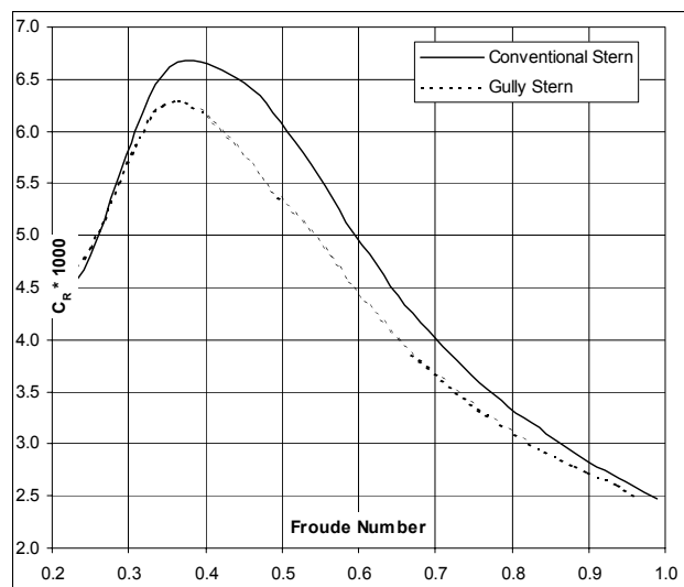
Figure 15 - C_R Vs F_N
