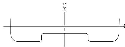
Fig 6 - Modified ‘Gullied’ Transom – Raised Centre Jets
