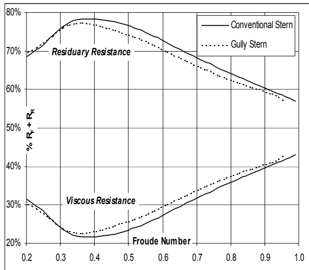
Figure 16 - % R_F & % R_R Vs F_N
