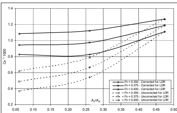
Figure 4 – C_R Vs A_T/A_X
