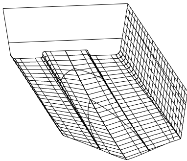
Figure 12 : Gully Stern
