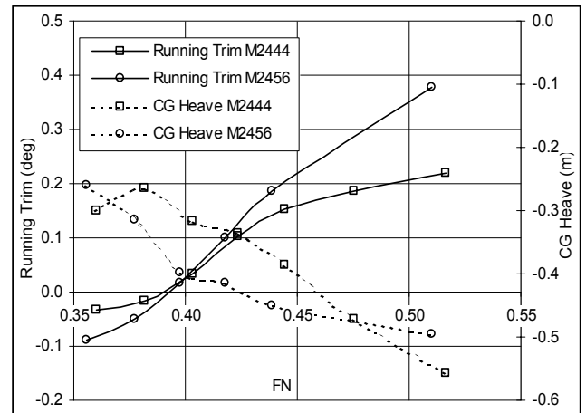
Figure 10 – Sinkage & Trim M2444 & M2456
