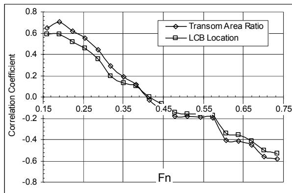
Figure 3 – Correlation Between C_R , A_T/A_X & LCB
