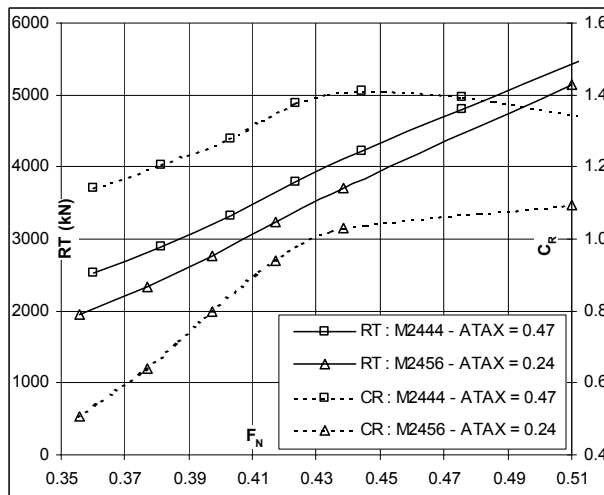
Figure 9 - RT & C_R Vs F_N
