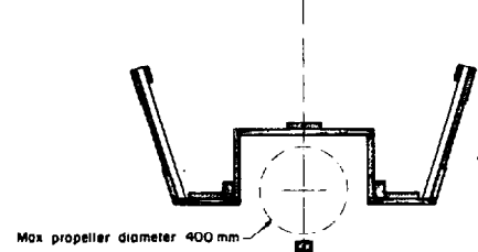
SECTION THROUGH TUNNEL
