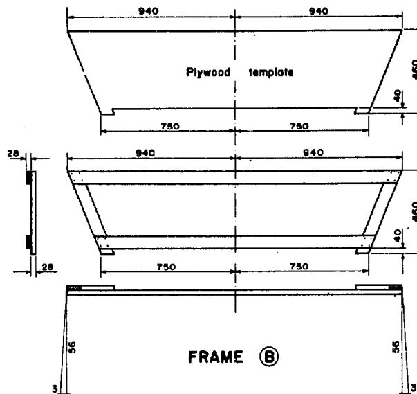
LOWER SIDE PLYWOOD
