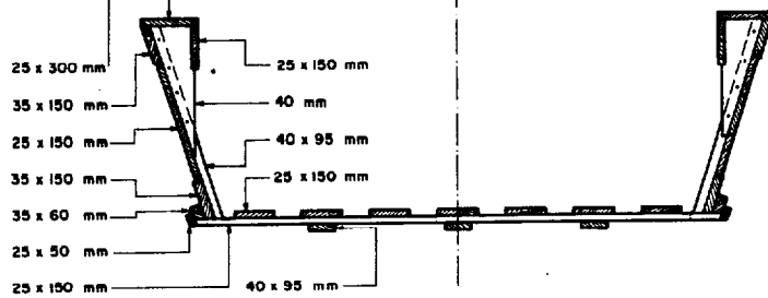
TYPICAL SECTION
